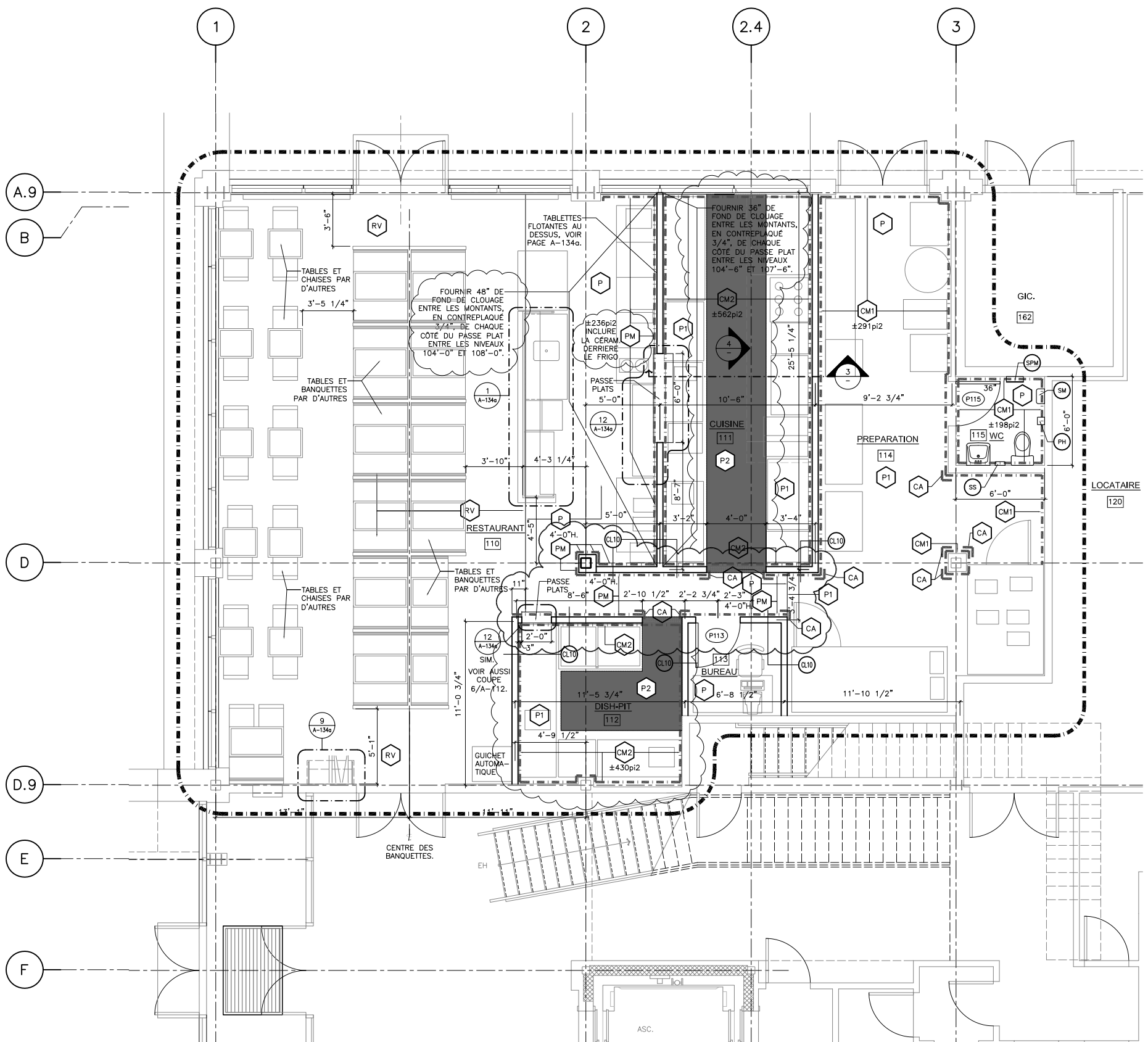
PLAN D'AMENAGEMENT RDC - RESTAURANT 1/4" = 1'-0"
